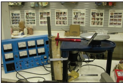
Torque test
